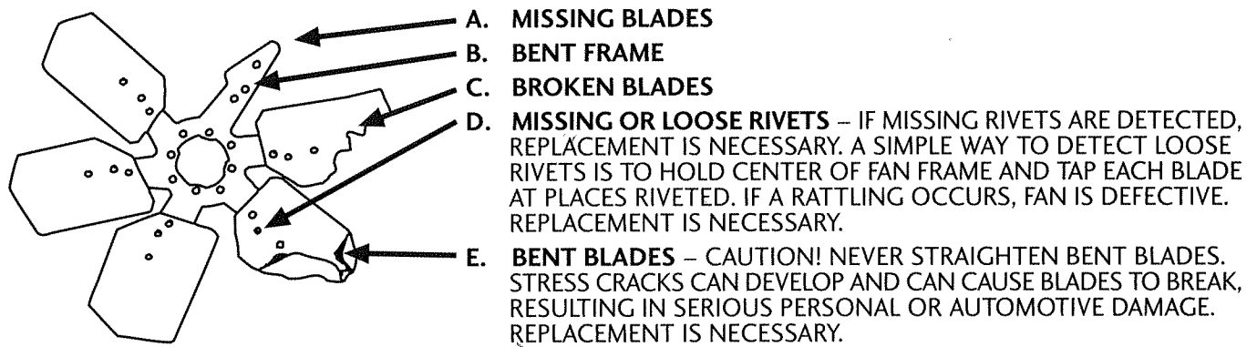
FIG. #1 IMPORTANT: ALWAYS REPLACE DAMAGED FANS Things To Look For When Inspecting Clutch Fan:
